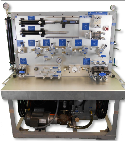
Double-Sided Hydraulic Trainer
